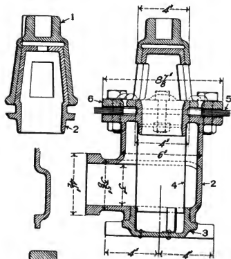
Figs. 4123-4128. Tank Valve.
